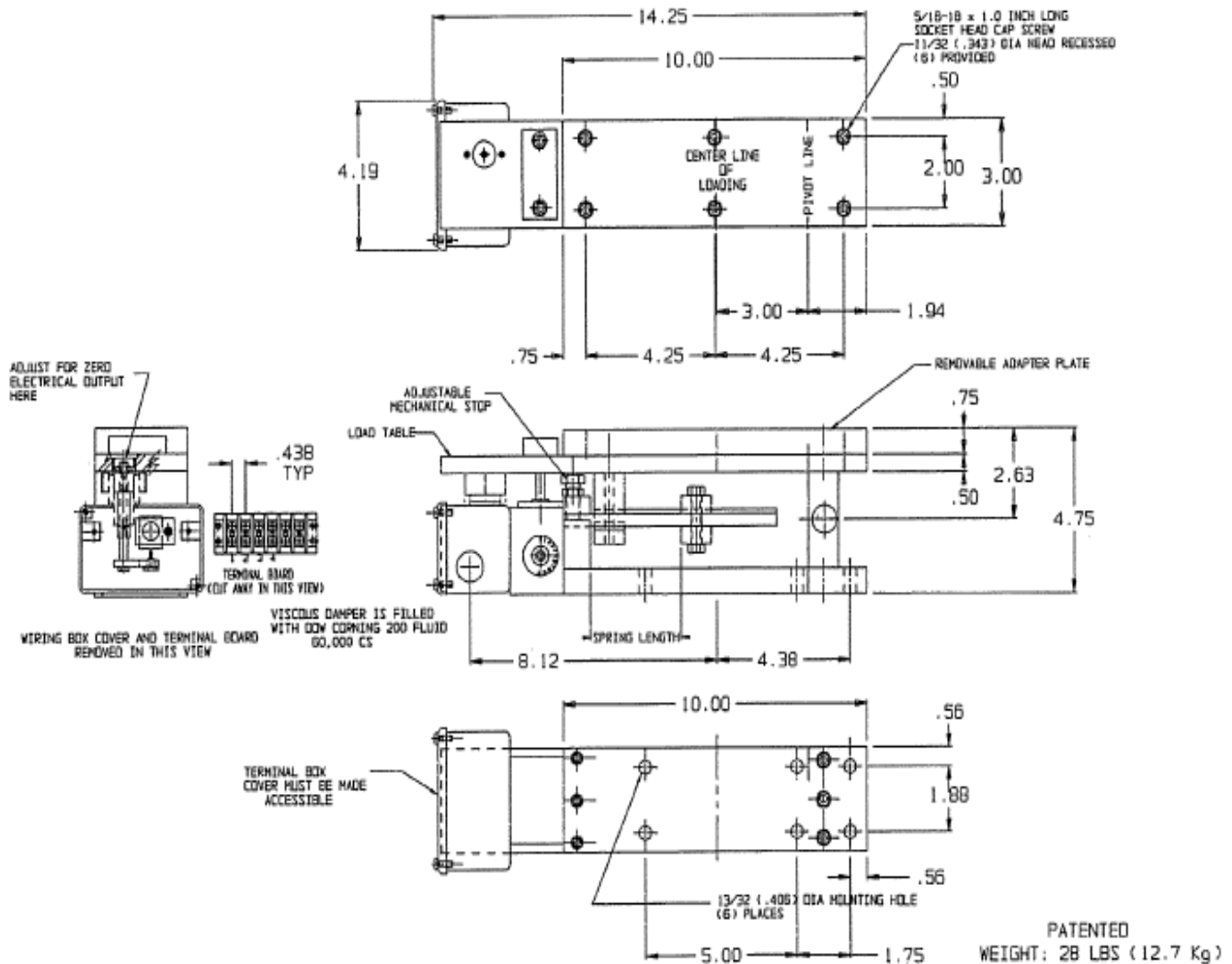
MODEL DST226-C SUPERLOADCELL
